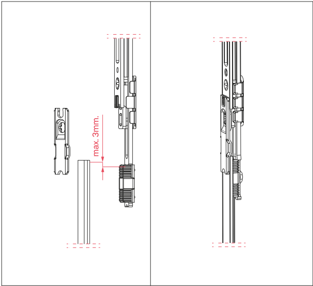
Manuel cut. Application of Corner Transmission Connecting Part.
