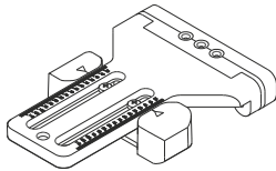
Jig for Turn Hinges "ART" • Product Code: 300020 • Hole Diameter 3 mm • Color - Red
